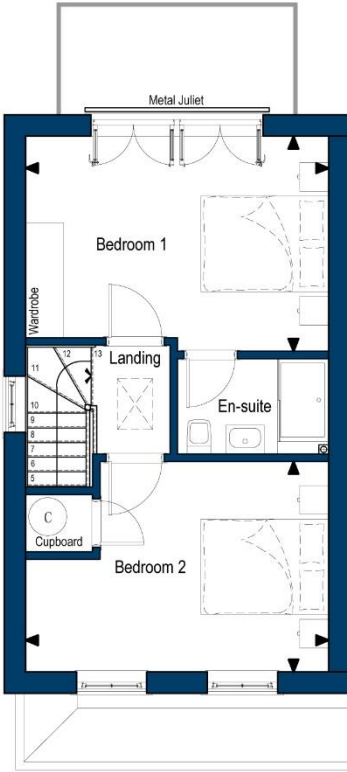
SECOND FLOOR Bedroom 1 4.75m x 3.37m (15'7" x 11'1") Bedroom 2 4.75m x 3.3m (15'7" x 10'10")
