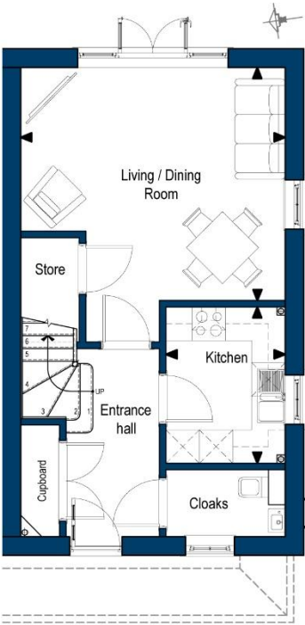
GROUND FLOOR Kitchen 2.8m x 2.14m (9'2" x 7'0") Living / Dining Room 4.75m x 4.17m (15'7" x 13'8")
