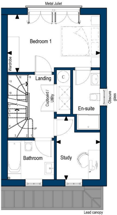
FIRST FLOOR Bedroom 1 4.75m x 2.93m (15'7" x 9'7") Study 3.21m x 2.24m (10'6" x 7'4")
