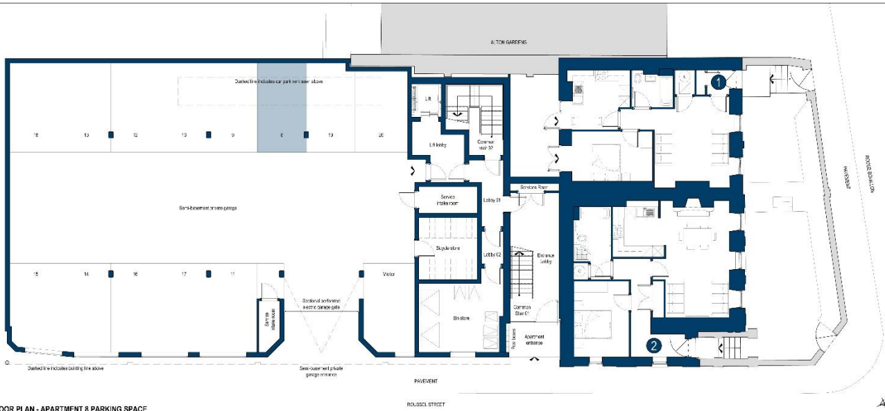
GROUND FLOOR PLAN - APARTMENT 8 PARKING SPACE
