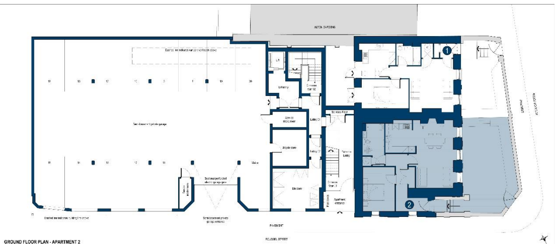
GROUND FLOOR PLAN - APARTMENT 2
